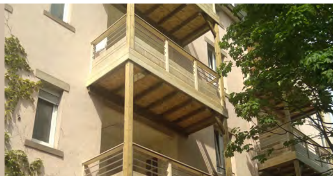
Terrasses multi-étages
